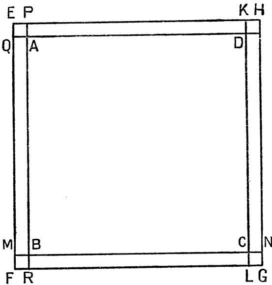
FIG. 5.—EVALUATION OF \sqrt{5000} (TALMUDIC METHOD).
